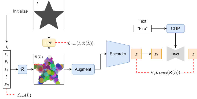
Fig. 6: Loss Function
