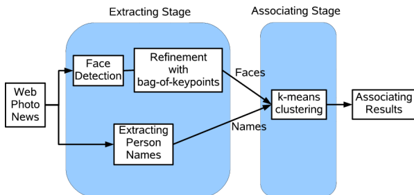
Figure 1. The processing flow of the proposed system.
